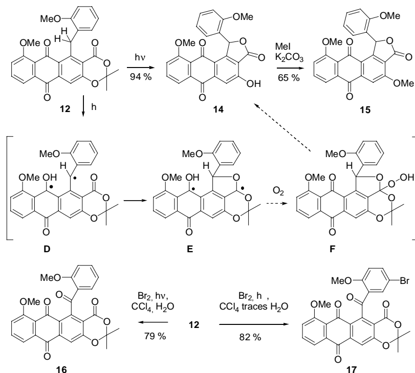
Scheme 4. Photooxidation of 1,3-dioxanaphthacene-4,6,11-trione 12 to the anthra[2,1- c ]furan 15 and bromination of 12 to the ketones 16 and 17 .
