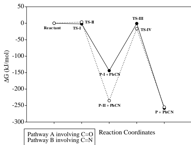
Figure 4. Free energy profile evaluated at the HF/3-21G* level for compound 13 .
