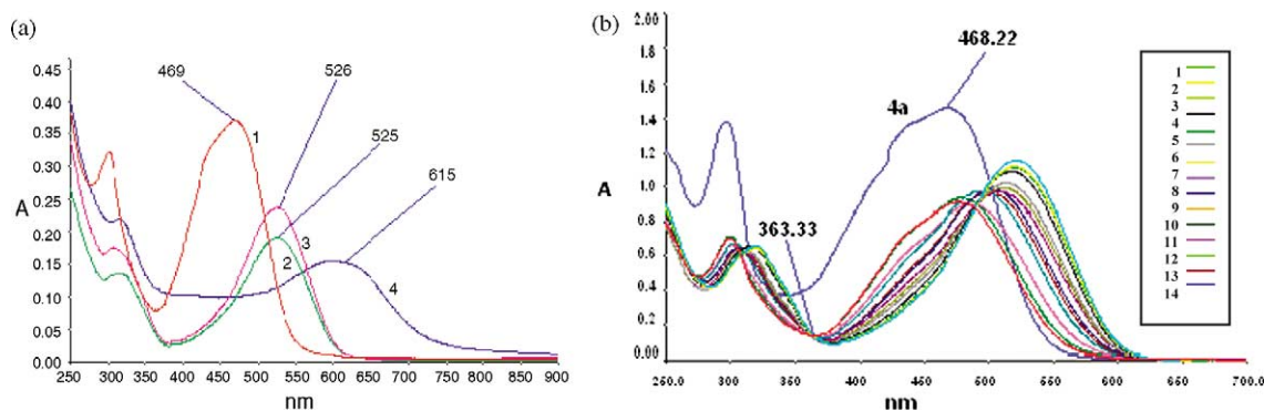
Figure 4. (a) UV-visible spectra of 10^{-4} M solution of 4a and shifts in its \lambda_{\text{max}} upon the addition of 10^{-4} M solutions of (2) \text{Cs}_2\text{CO}_3 , (3) \text{Rb}_2\text{CO}_3 and (4) \text{K}_2\text{PdCl}_4 in a Methanol–chloroform ( v/v = 1/1 ) cosolvent; (b) changes in the UV-visible spectra of 4a upon titration by \text{Cs}_2\text{CO}_3 in a methanol–chloroform ( v/v = 1/1 ) cosolvent where the concentration of \text{Cs}_2\text{CO}_3 (1) 1 \times 10^{-4} (2) 2 \times 10^{-4} (3) 3 \times 10^{-4} (4) 4 \times 10^{-4} (5) 5 \times 10^{-4} (6) 6 \times 10^{-4} (7) 7 \times 10^{-4} (8) 8 \times 10^{-4} (9) 9 \times 10^{-4} (10) 1 \times 10^{-3} (11) 2 \times 10^{-3} (12) 3 \times 10^{-3} (13) 4 \times 10^{-3} (14) 5 \times 10^{-3} .
