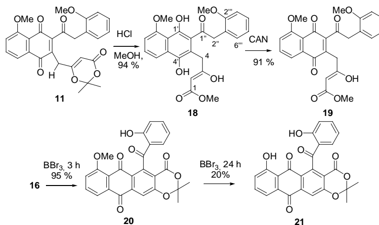
Scheme 5. Methyl ester and methyl ether cleavage of 11 and 16 using HCl/MeOH or boron tribromide.
