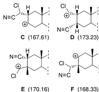
Figure 2. The intermediate carbocationic species C , D and E , F postulated in the Beckmann rearrangement of \alpha -chlorooximes 16 and 20 , respectively. AM1 enthalpies are in kcal/mol.
