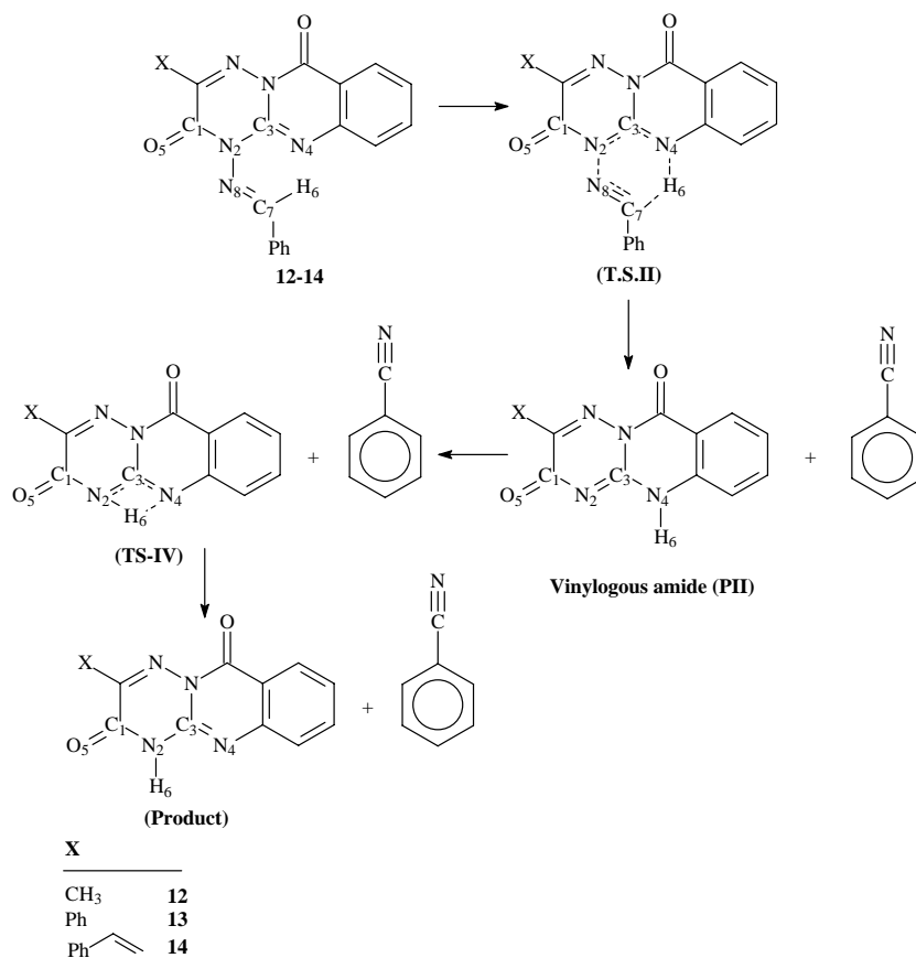
Scheme 8. Pathway B involving (C=N).
