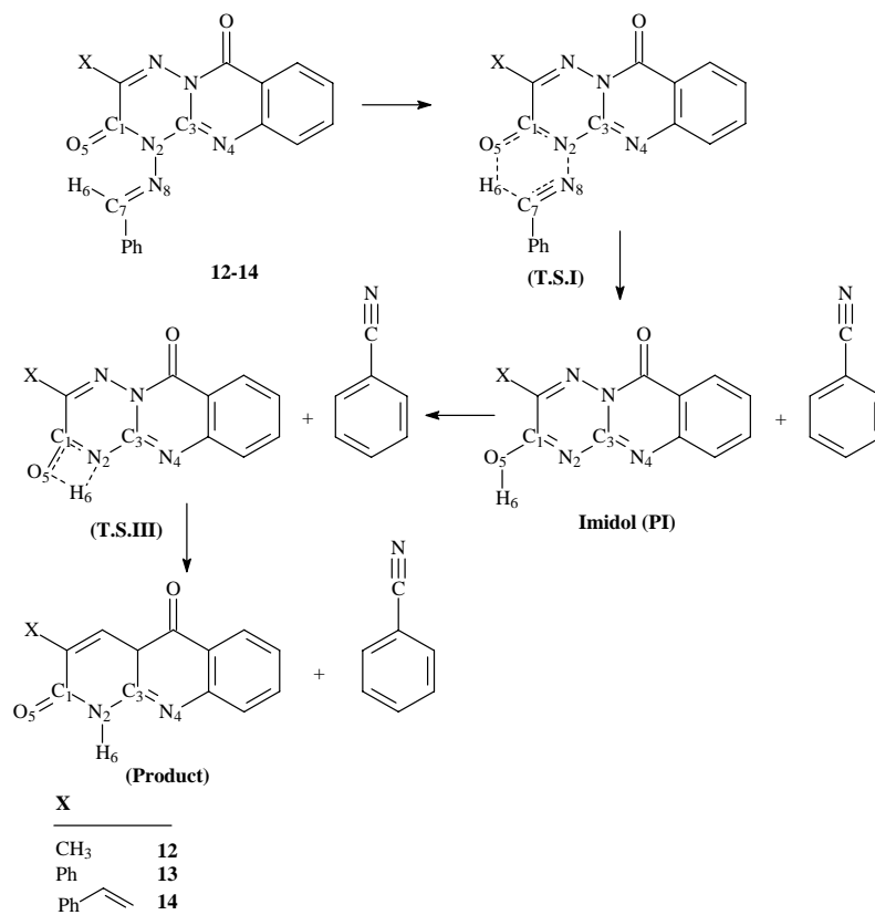
Scheme 7. Pathway A involving the (C=O).
