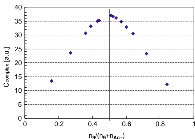
Figure 2. Job's plot for the 9 + Bu 4 N + AcO - system, ( 1 H NMR, 300 MHz, 298 K, CHCl 3 :CH 3 CN=4:1 v/v).
