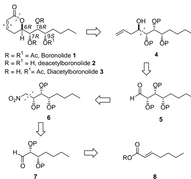
Scheme 1. Retrosynthetic approach to (+)-boronolide.
