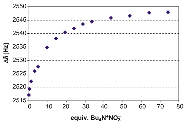
Figure 1. 1 H NMR titration of 9 with Bu 4 N + NO 3 - (300 MHz, 298 K, CHCl 3 /CH 3 CN=4:1 v/v).
