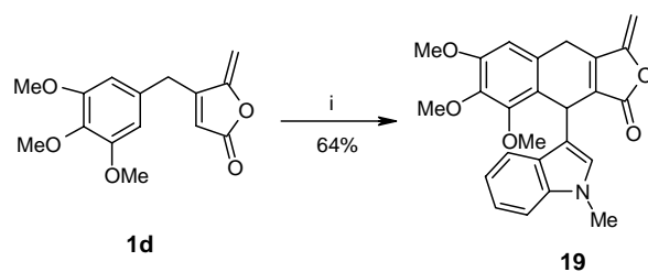
Scheme 6. Reagents and conditions: (i) (a) N -Methyl indole-3-carboxaldehyde, LDA, THF, -78\text{ }^{\circ}\text{C} ; (b) Dilute acetic acid.
