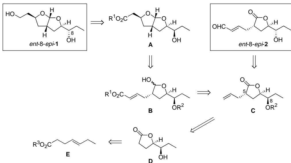
Scheme 1. Retrosynthetic analysis of ent-8-epi-1 and ent-8-epi-2 .
