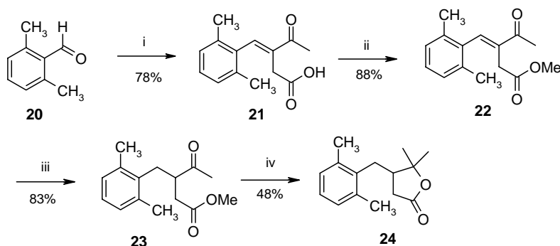
Scheme 7. Reagents and conditions: (i) aq. NaOH, methanol, -10\text{ }^{\circ}\text{C} , 4–5 h; (ii) \text{CH}_2\text{N}_2 , methanol, rt; (iii) \text{H}_2 , Pd/C, methanol, rt; (iv) \text{CH}_3\text{MgI} , ether, -78\text{ }^{\circ}\text{C} , 5 h.
