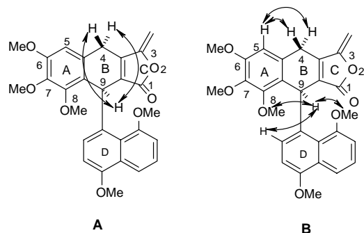
Figure 1. Selected COSY and NOESY correlations.
