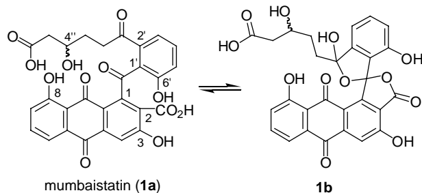
Chart 1. Structure of the open chain ( 1a ) and cyclic hemiacetal form ( 1b ) of mumbaistatin. 1
