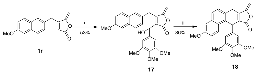
Scheme 5. Reagents and conditions: (i) 3,4,5-Trimethoxy benzaldehyde, LDA, THF, -78\text{ }^{\circ}\text{C} ; (ii) TFA, \text{CH}_2\text{Cl}_2 , rt.
