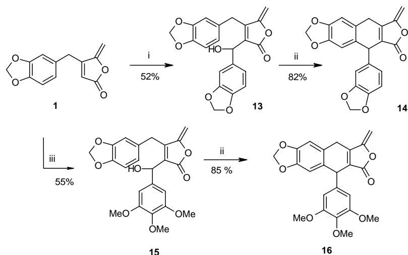
Scheme 4. Reagents and conditions: (i) 3,4-Methylene dioxybenzaldehyde, LDA, THF, -78\text{ }^{\circ}\text{C} ; (ii) TFA, \text{CH}_2\text{Cl}_2 , rt; (iii) 3,4,5-Trimethoxybenzaldehyde, LDA, THF, -78\text{ }^{\circ}\text{C} .
