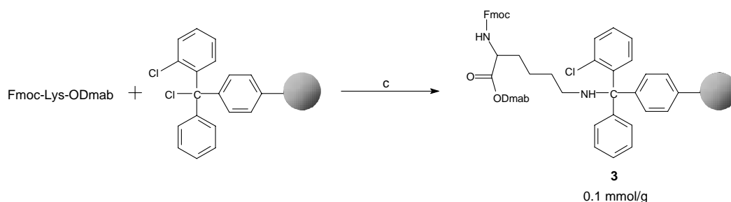
Scheme 3. Anchoring of Fmoc-Lys-ODmab to the 2-chlorotrityl resin. (c) DIEA, THF, rt, 5 h.
