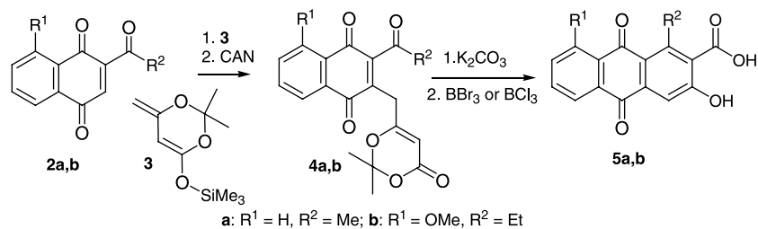
Scheme 1. Construction of contiguously 1,2,3-substituted anthraquinones 5a 6 and 5b . 8
