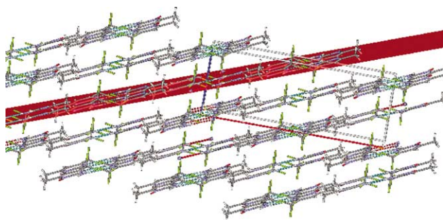
Figure 3. Crystal packing of 1b .
