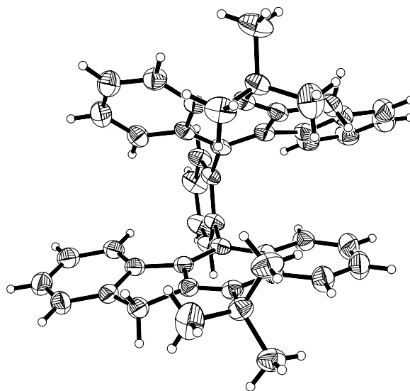
Figure 1. Perspective view of the molecular structure of 12a with the thermal ellipsoids scaled to enclose 30% probability.
