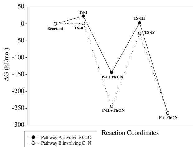
Figure 3. Free energy profile evaluated at the HF/3-21G* level for compound 12 .
