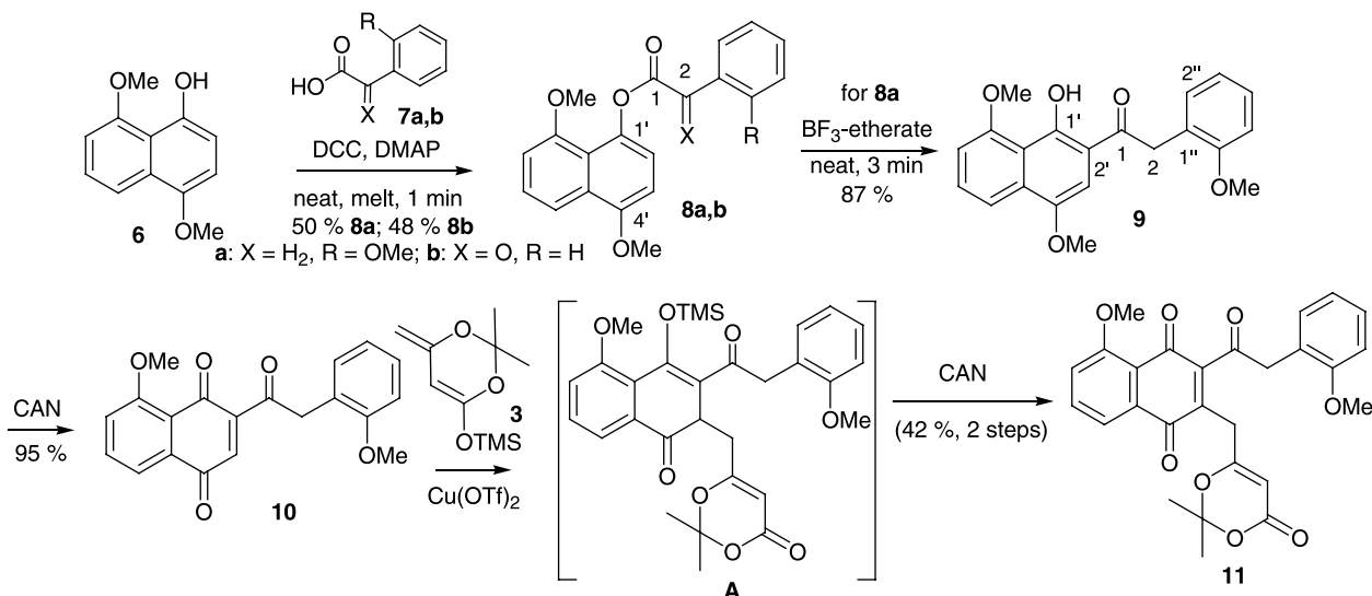
Scheme 2. Construction of the 2,3-bis-substituted naphthoquinone 11 .
