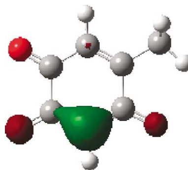
Figure 1. HOMO of 2-hydroxy-5-methyl-1,4-benzoquinone calculated at the HF/6-31+G(d,p) level using PCM to model the effects of the solvent medium.
