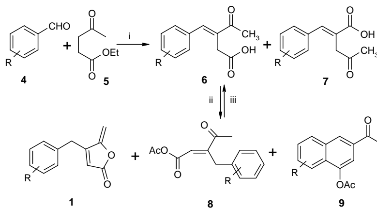
Scheme 2. Reagents and conditions: (i) Aq. NaOH, ethanol, -10\text{ }^{\circ}\text{C} , 4–5 h, (7, 80–95%); (ii) Anhydr. NaOAc, \text{Ac}_2\text{O} , 80\text{ }^{\circ}\text{C} , 3 h; (iii) Aq. NaOH, ethanol, rt, 2–3 h.
