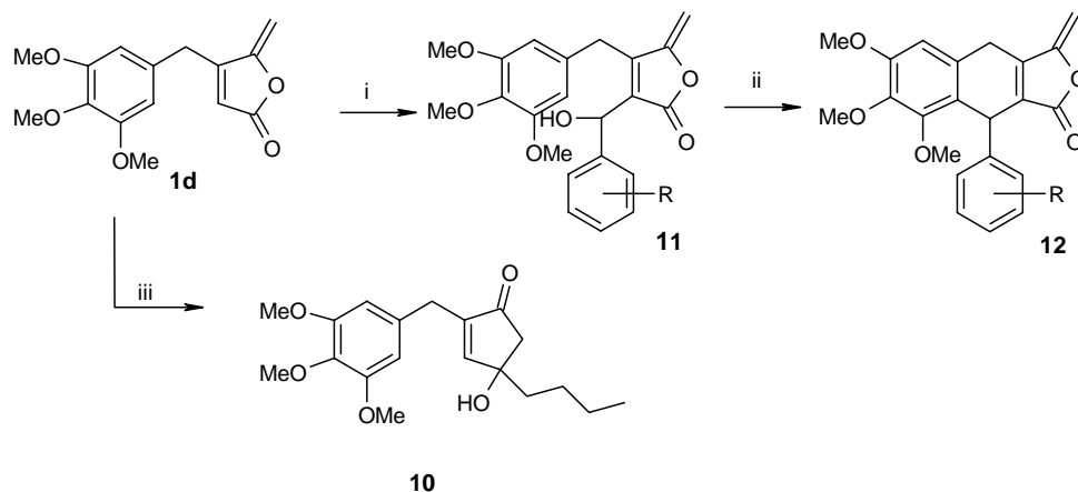
Scheme 3. Reagents and conditions: (i) LDA, substituted arylaldehydes, -78\text{ }^\circ\text{C} ; (ii) TFA, dichloromethane, rt; (iii) n -BuLi, -78\text{ }^\circ\text{C} , 40%.
