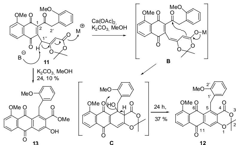
Scheme 3. Cyclization of the disubstituted naphthoquinone 11 to the 1,3-dioxanaphthacene-4,6,11-trione 12 and the methyl ester 13 .
